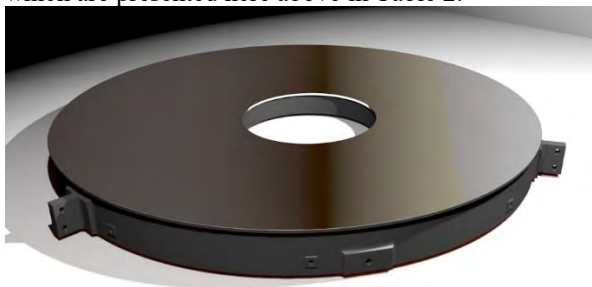
Figure 5. Euclid M1 design, optical face
